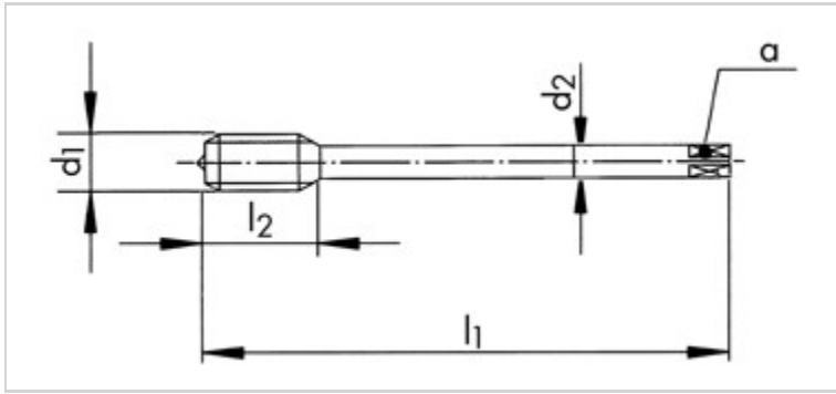
TECHNICAL DRAWING
