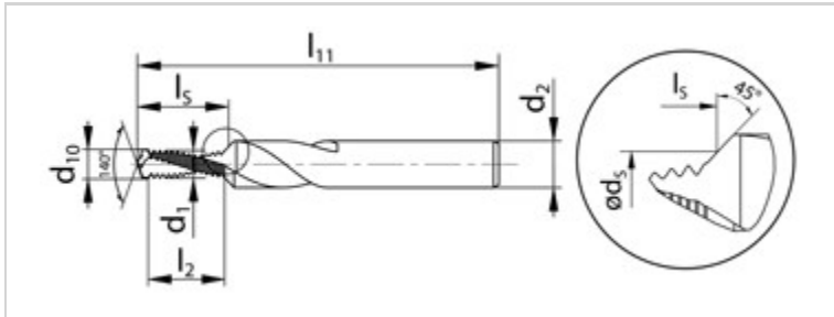
TECHNICAL DRAWING
